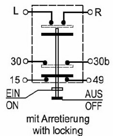
Circuit diagram
